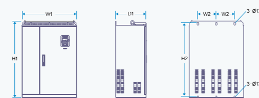
220-350kW Wall mounting Installation diagram
