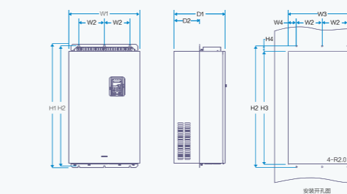
132-200kW Flange mounting Installation diagram
